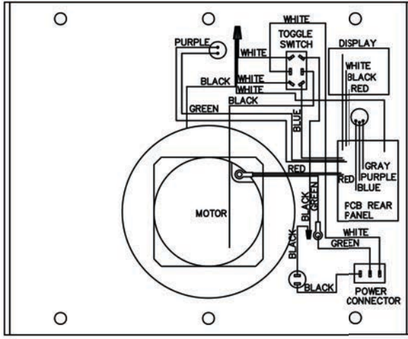
WIRING DIAGRAM
