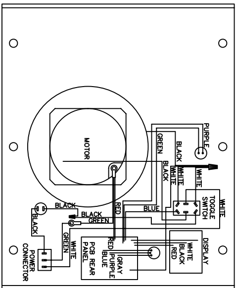
MODEL 1050VR
