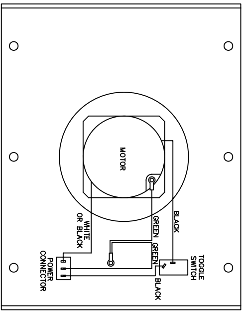
WIRING DIAGRAM
