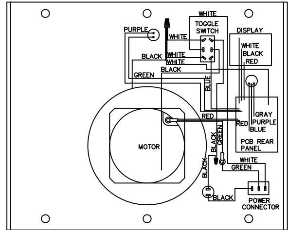
WIRING DIAGRAM
